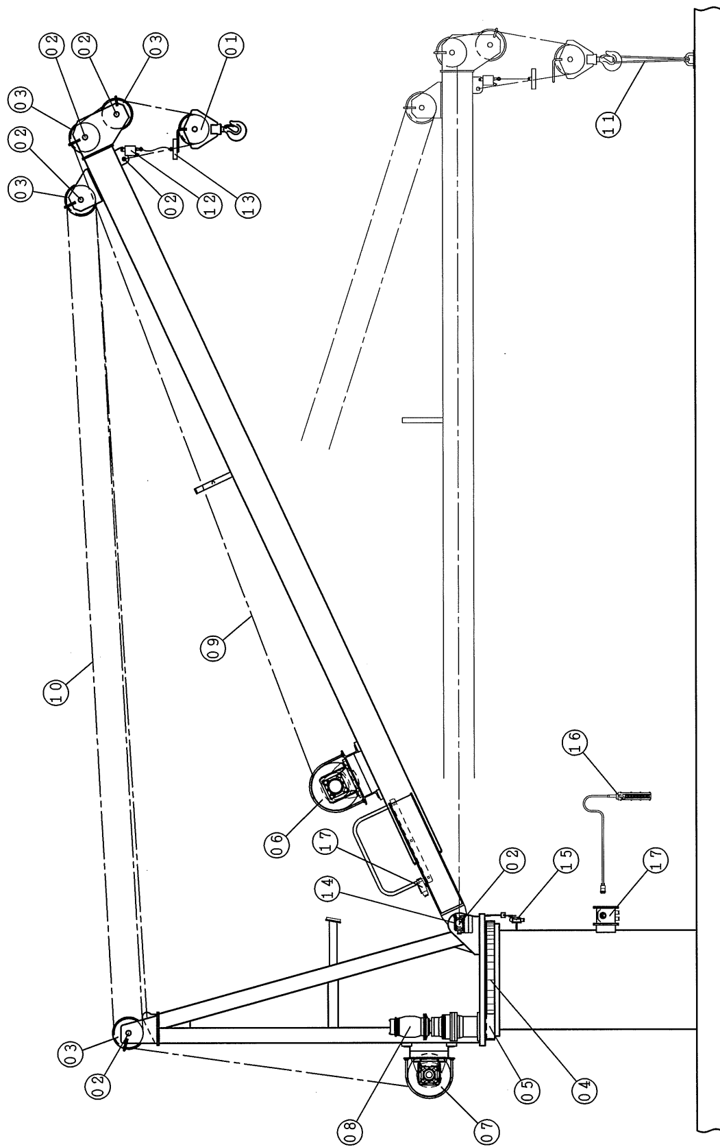
交換部品の配置 (型式: RD-□□PL) LAYOUT OF THE REPLACEMENT PARTS (MODEL: RD-□□PL)
